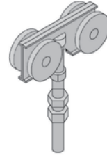
0200 HANGER (200kg) 0460 HANGER (400/600kg) 1000M HANGER (1000kg) FOR STEEL DOORS
