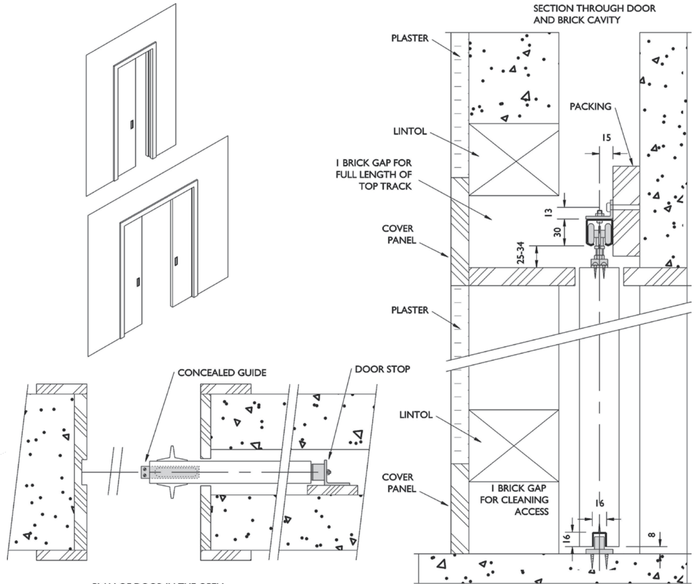
PLAN OF DOOR IN THE OPEN POSITION IN THE BRICK CAVITY. NOT TO SCALE
